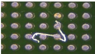
Lint contamination
